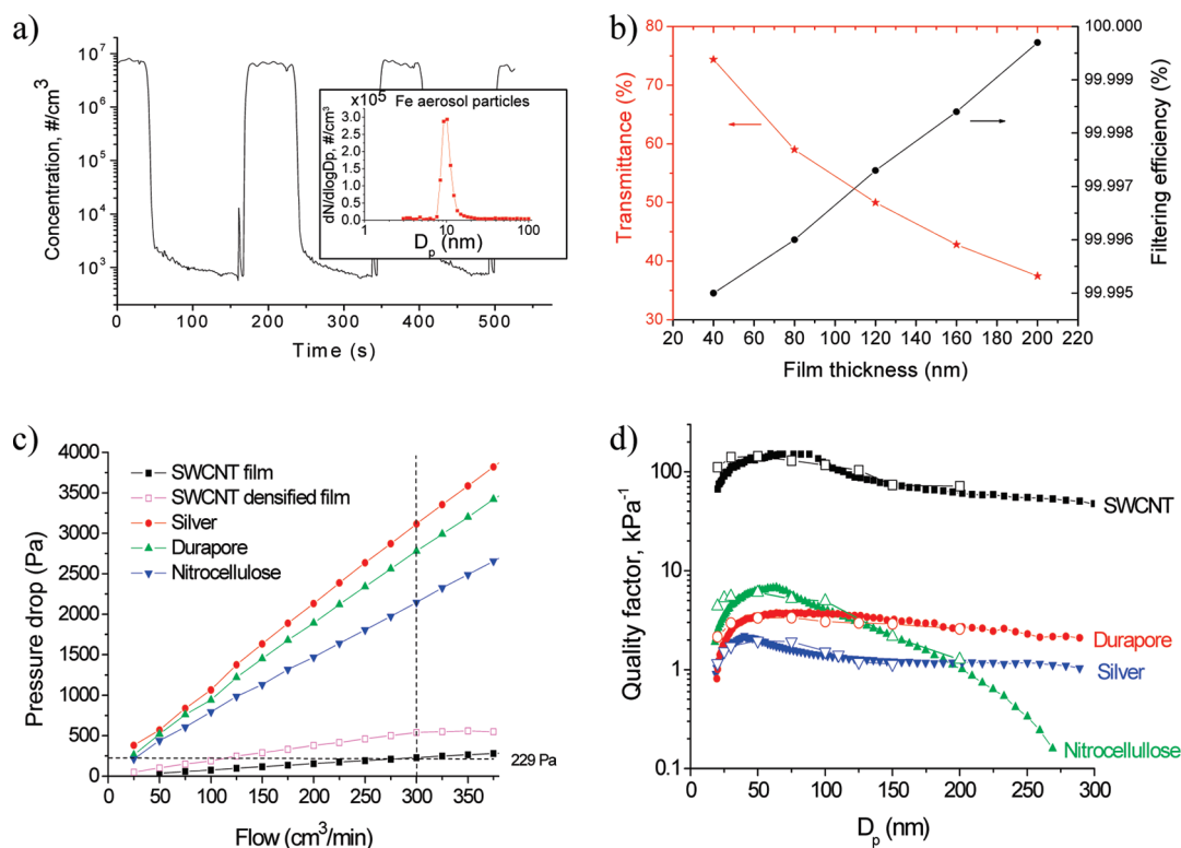
Figure 2. FSF air filter characterization. (a) Change in 11 nm sized Fe particle concentration measured by a particle counter when the flow passed alternately through a filter and a bypass. The film is 70 nm thick with transmittance of 64% and filtering efficiency of 99.99%. The inset shows the number size distribution of the Fe particles used for the efficiency test. (b) Thickness dependence of transmittance and of collection efficiency for 44 nm \gamma -Fe 2 O 3 particles. (c) Flow rate dependence of pressure drop for 120 nm thick SWCNT films and various commercial filters. (d) Dependence of the filter quality factor on the particle size for commercial filters and a 120 nm thick SWCNT film. The solid and open symbols show results obtained by two independent measurement techniques, namely, scanning over the entire particle size range studied and at fixed particle sizes.
