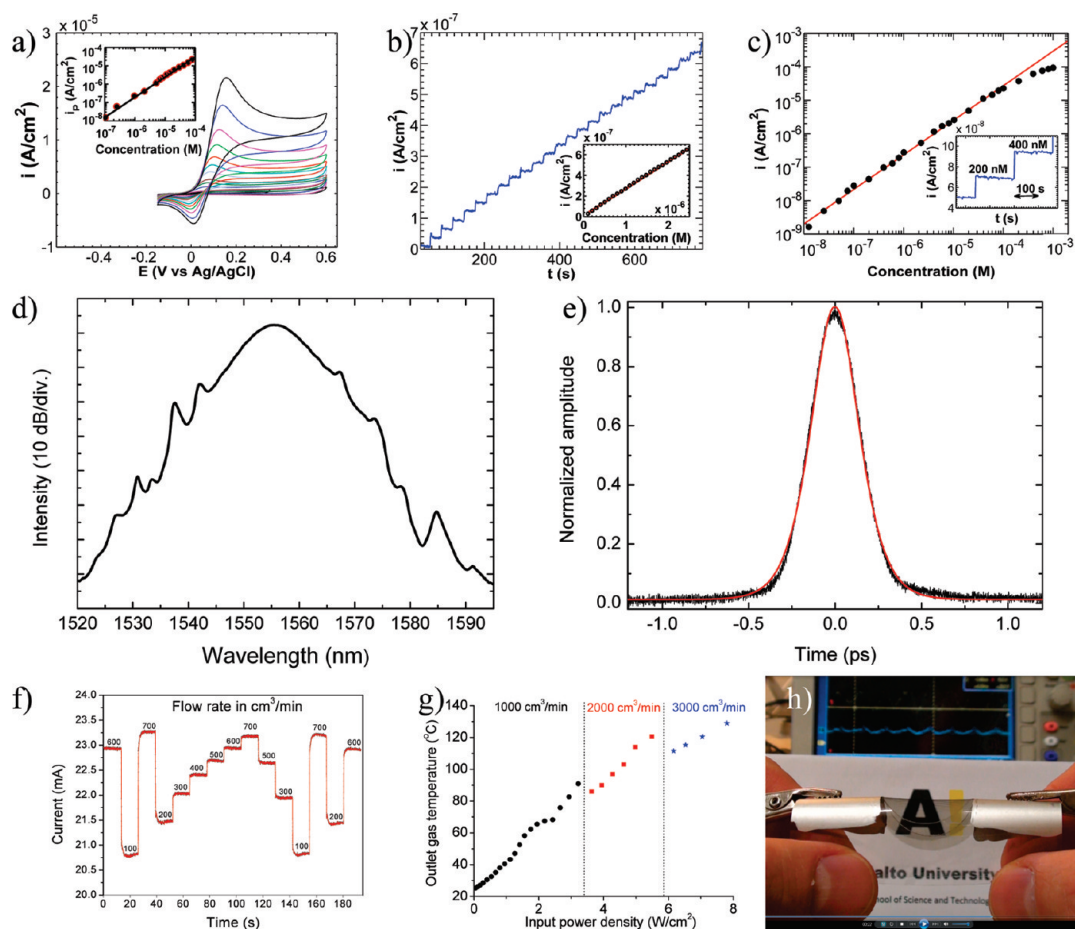
Figure 4. FSFs for various applications. (a–c) Chemical sensor. (a) Cyclic voltammograms of an FSF electrode in solutions with increasing concentrations of dopamine (from 0.1 to 80 \mu\text{M} ). Scan rate: 50 \text{mV s}^{-1} . The inset shows the peak current versus dopamine concentration and the corresponding linear fit. (b) Amperometric response of an FSF electrode to successive additions of 100 nM dopamine at an applied potential of +0.2 V versus Ag/AgCl. The inset shows the corresponding calibration plot. (c) Calibration plot for the amperometric response of an FSF electrode at an applied potential of +0.2 V versus Ag/AgCl in solutions with increasing dopamine concentration. The inset shows the stability of the SWCNT sensor at the operating potential at very low dopamine concentrations. The supporting electrolyte was a 0.1 M PBS with pH = 7. (d,e) Laser absorber: (d) optical spectrum and (e) autocorrelation trace with a \text{sech}^2 fit for an all-fiber mode-locked Er laser. The spectral width is \sim 11.3 nm and the corresponding pulse width is 220 fs. (f) Gas flowmeter. Electrical current through the FSF at different nitrogen flow rates. (g) Gas heater. Temperature of outflowing gas versus input power density at different flow rates. (h) Thermoacoustic speaker based on SWCNTs. Demonstration of its flexibility.
